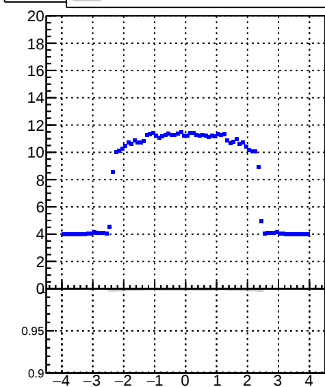
mean hit tracking_lters01LST_DNN_1000events
