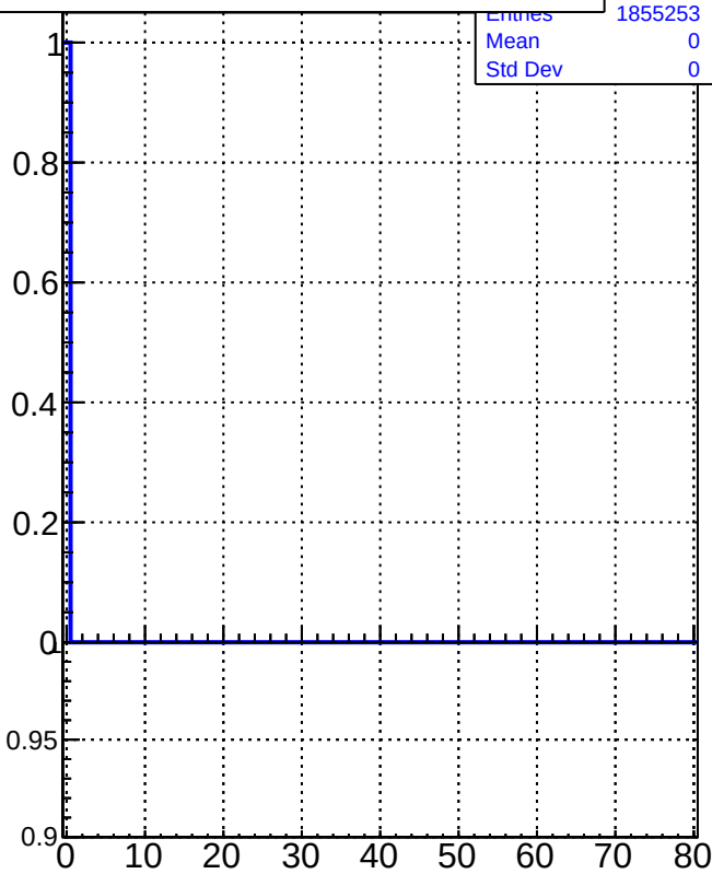
tracking_iters01LST_DNN_1000events
