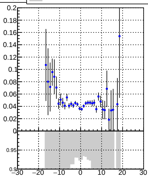
Efficiency vs. tracking_iters01LST_DNN_1000events
