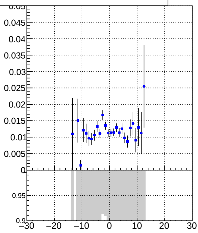
tracking_iters01LST_DNN_1000events
